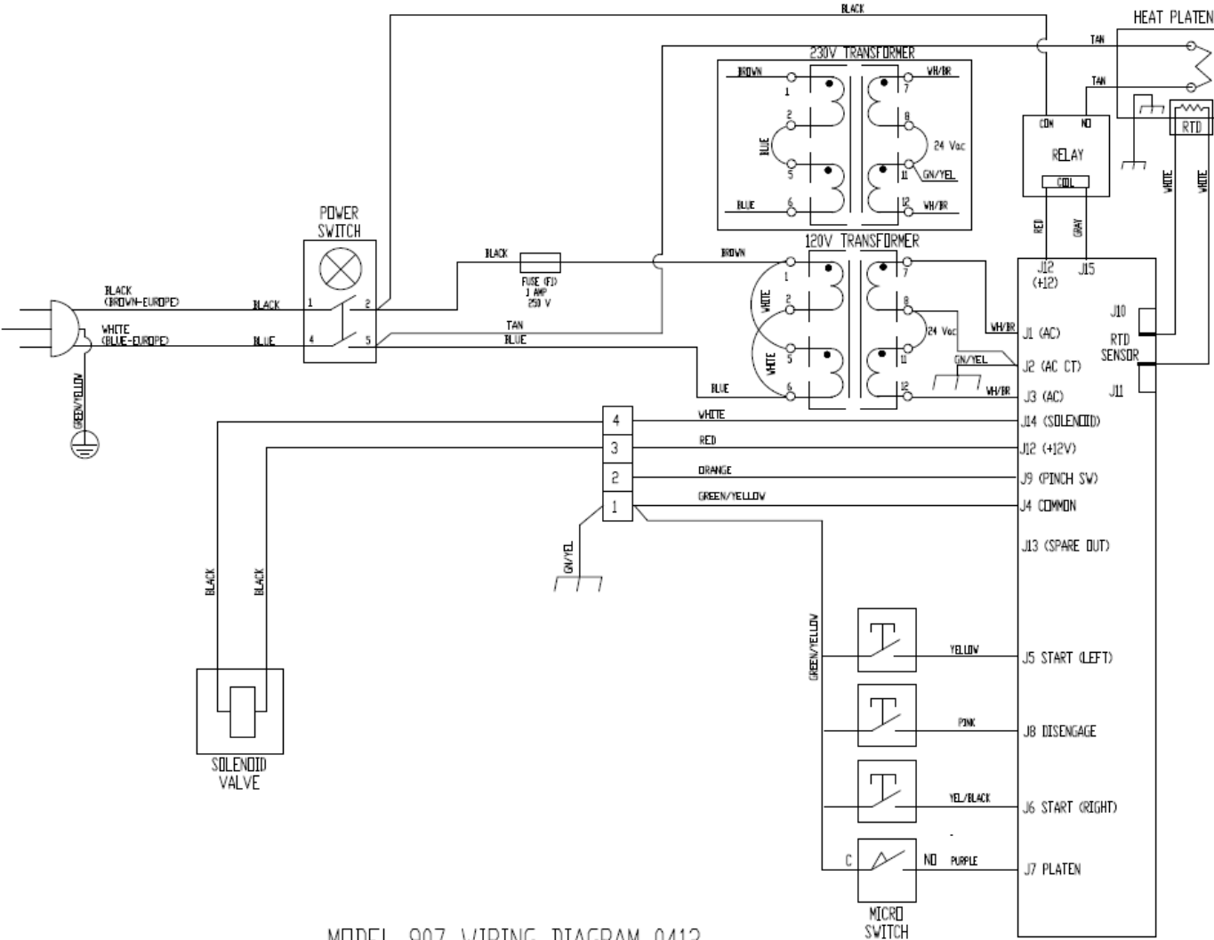
MODEL 907 WIRING DIAGRAM 0412
